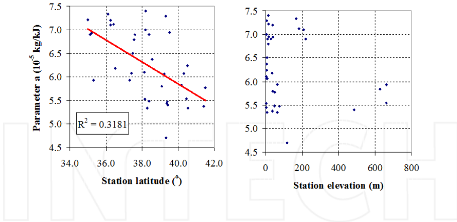
Figure 4. Scatter plots of parameter a (eq. 17) vs. latitude and elevation
